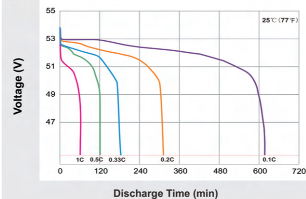
Discharge Time in relation to Discharge Rate
