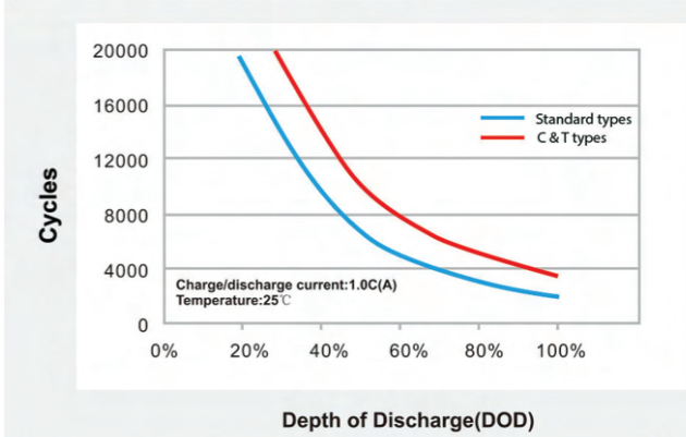
Depth of Discharge vs Cycle Life
